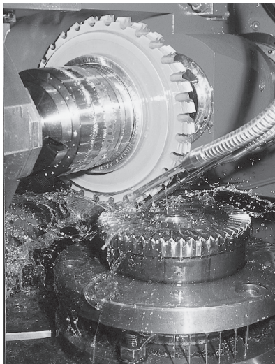
CNC machining of a PowerTRUE right-angle gear
