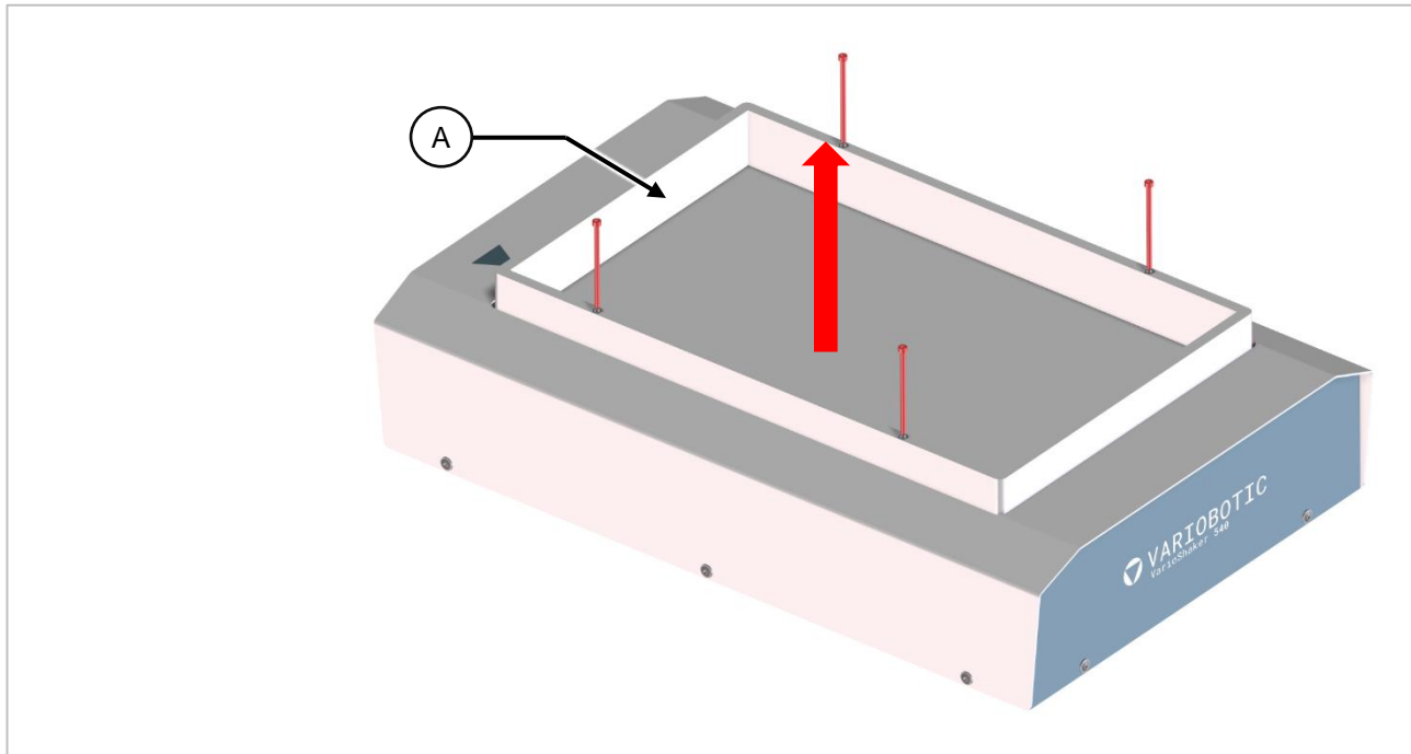
figure 4.3: Changing the vibration plate
