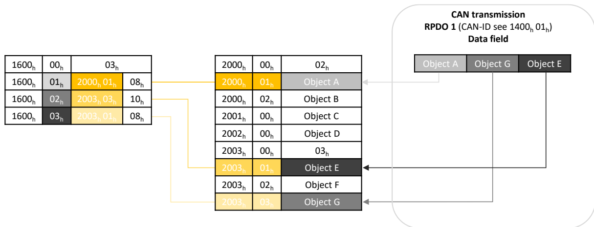
Figure 15 - RPDO mapping
