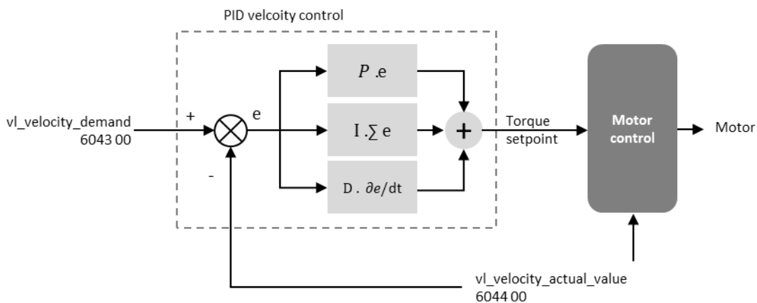
Figure 27 – Controller synoptic
